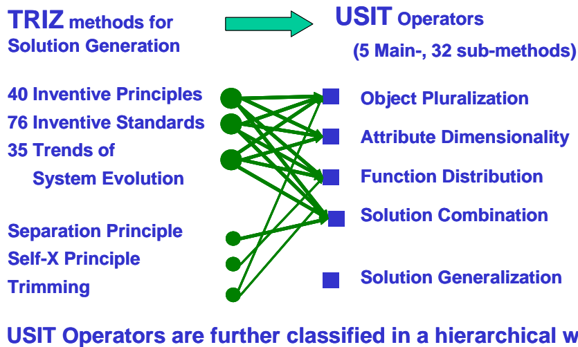
Fig. 6. Reorganizing all the TRIZ solution generation methods into the USIT Operators
