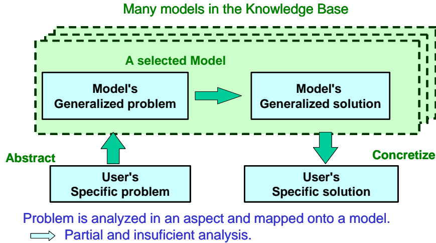
Fig. 12. Conventional 'Four-Box Scheme' for creative problem solving, i.e. the basic scheme in science and technology as well as in TRIZ
